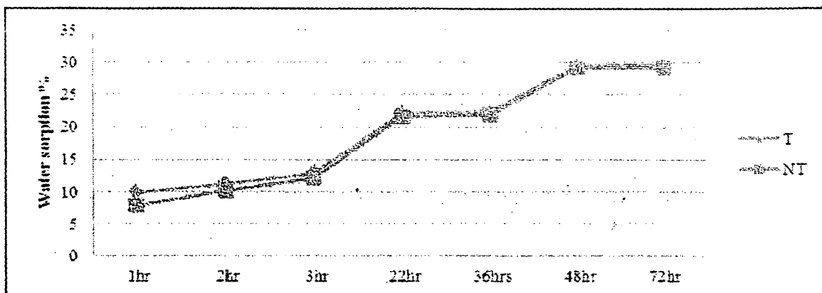
Figure 3. Water sorption behaviour of Tapped (T) and Non-tapped (NT) Kithul flour vs time
