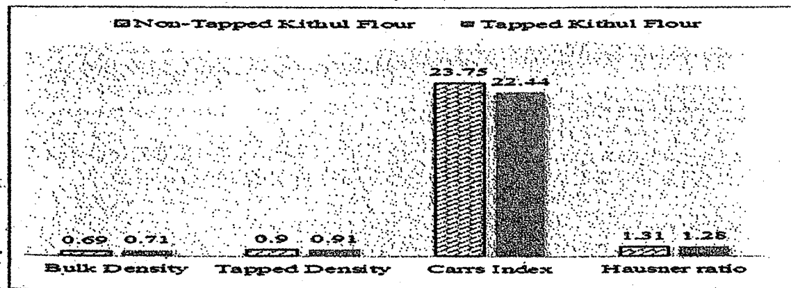
Figure 2 Comparison of Density of Tapped (T) and Non-tapped (NT) Kithul flour
