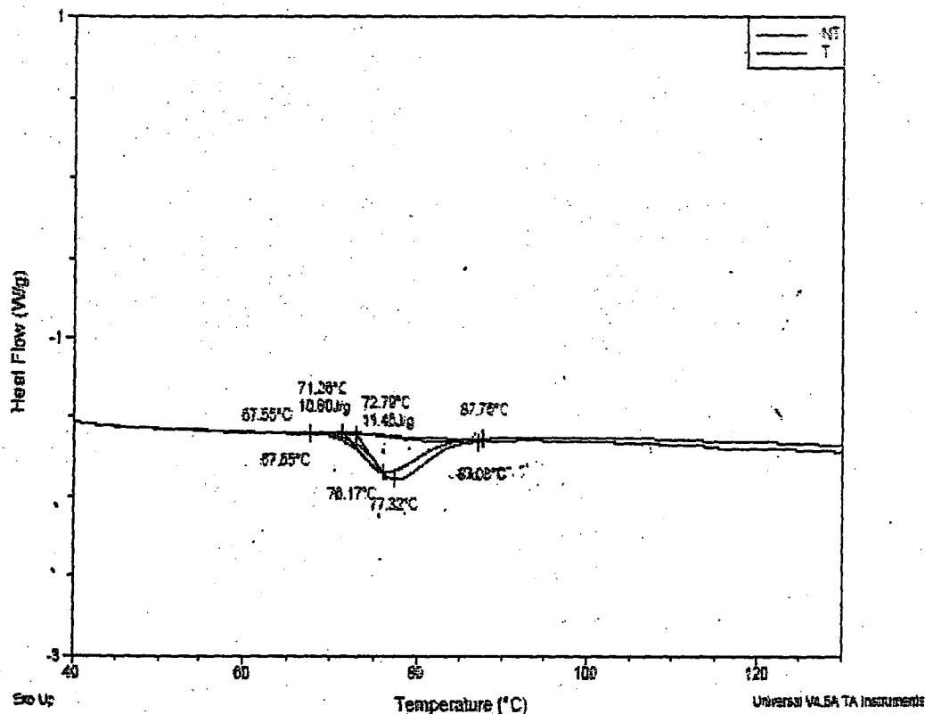
Figure 4 Gelatinization DSC curves of Kithul flour of Tapped (T) and non-tapped (NT)
